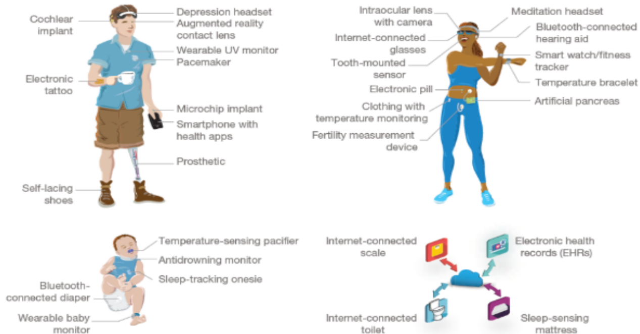
FIGURE 1 IoB Examples
